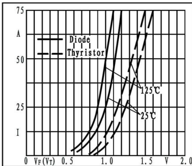
Fig2. Forward characteristics
