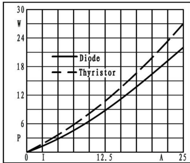
Fig3. Power dissipation
